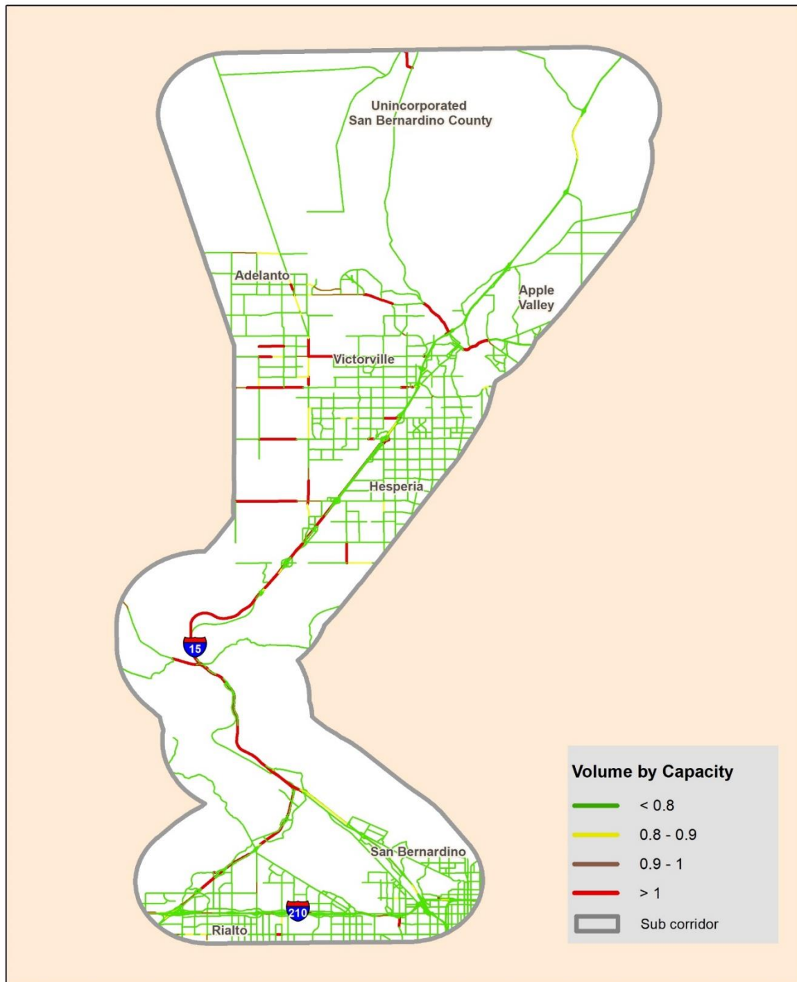
Figure 5.8 | Future 2040 Traffic Conditions—AM Victorville to San Bernardino Sub-Corridor
