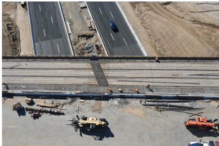
Crews prepare the I-215 Placentia Ave. bridge for an upcoming concrete pour.
