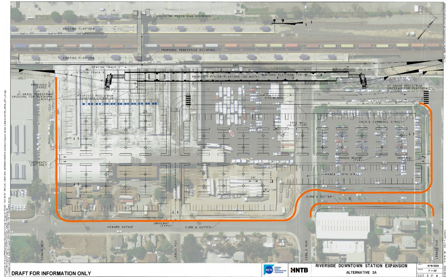
Figure 2-7. Build Alternative with Traffic Circulation and Parking Option 3A
