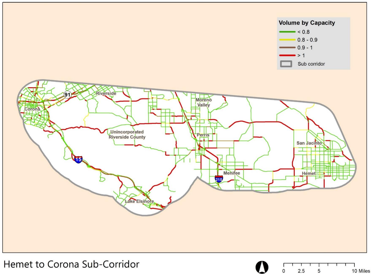
Figure 5.90 | Future 2040 Traffic Conditions—PM Hemet to Corona Sub-Corridor
