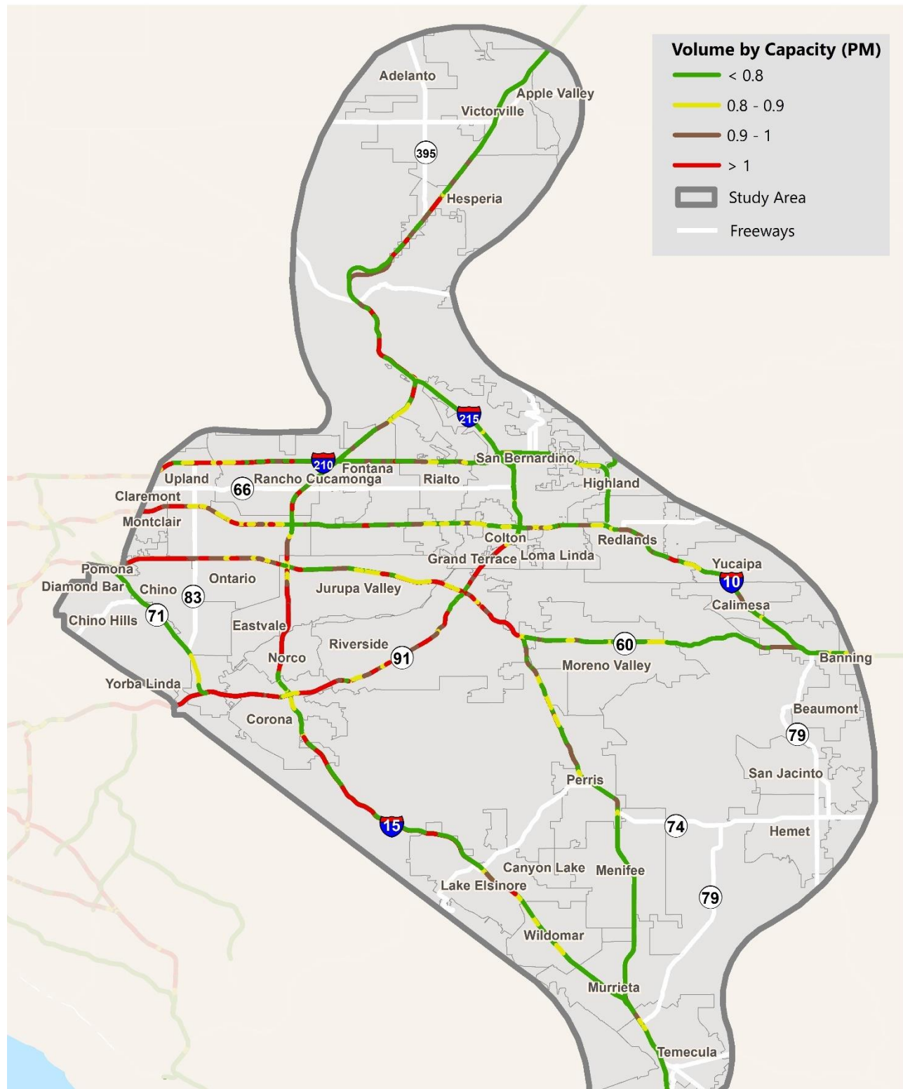
Figure 3.36 | PM Peak Hour Volume/Capacity Ratio
