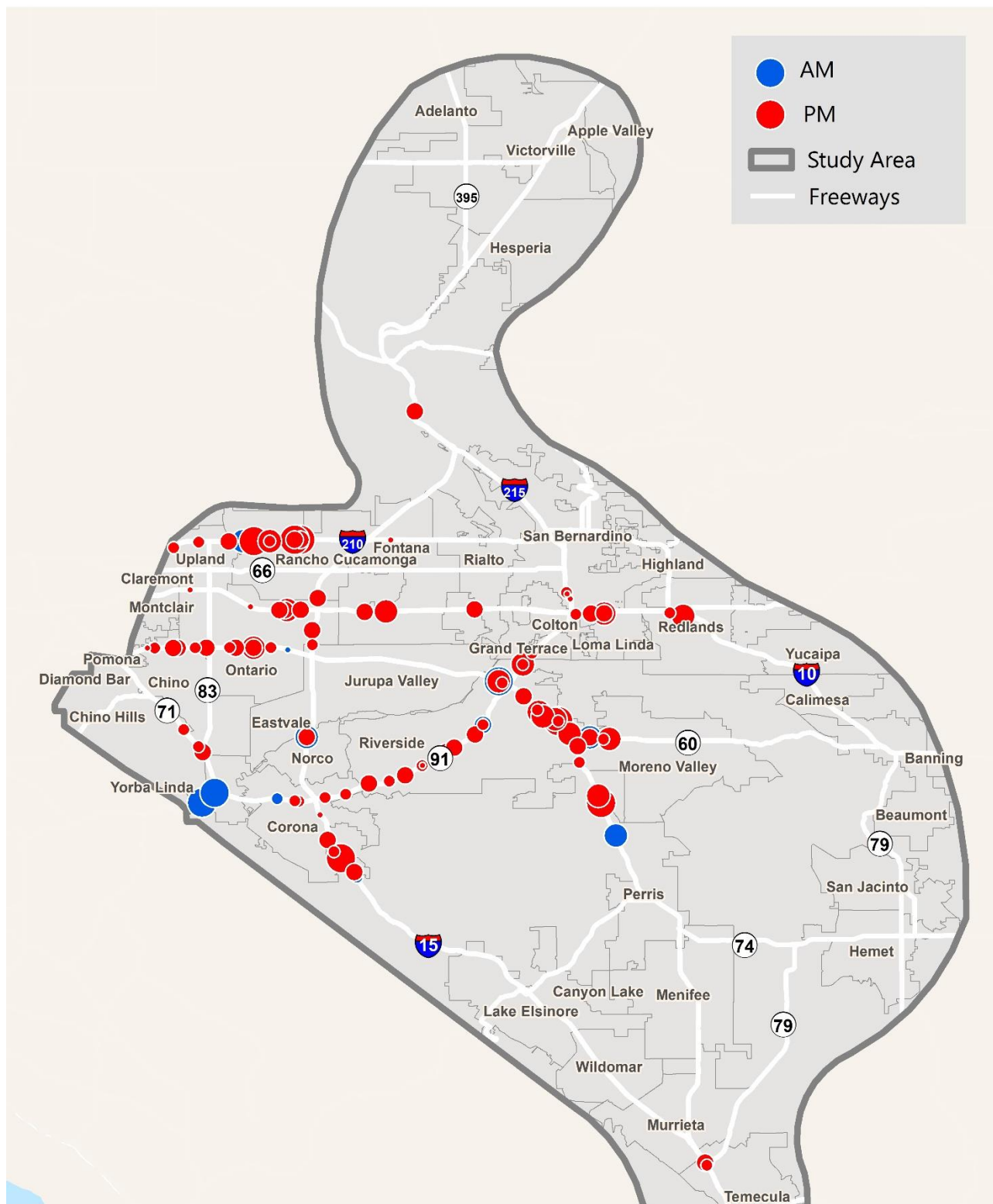
Figure 3.37 | Top Bottlenecks
