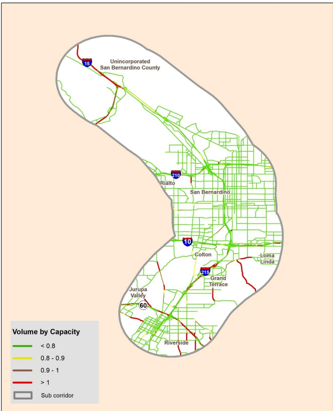
Figure 5.17 | Future 2040 Traffic Conditions—AM San Bernardino to Riverside Sub-Corridor
